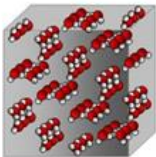
H 2 O (s)
