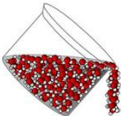
H 2 O (l)
