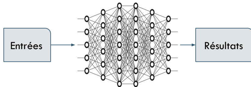
Machine Learning
