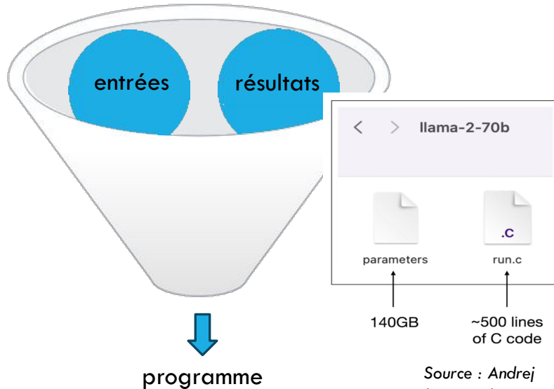
Machine Learning
